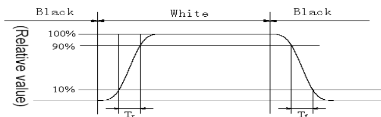
Fig4. Response Time Testing( T_a=25^{\circ}\text{C} )
