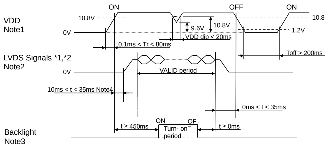
Figure 5.4.1 LCD power on/off
