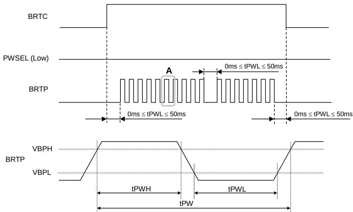
Figure 5.3.1 BRTP timing
