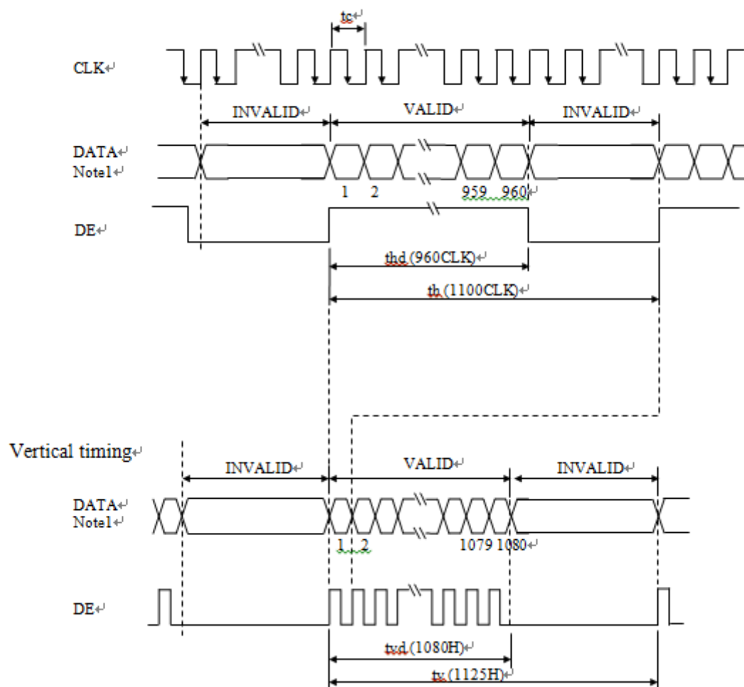
Horizontal timing
