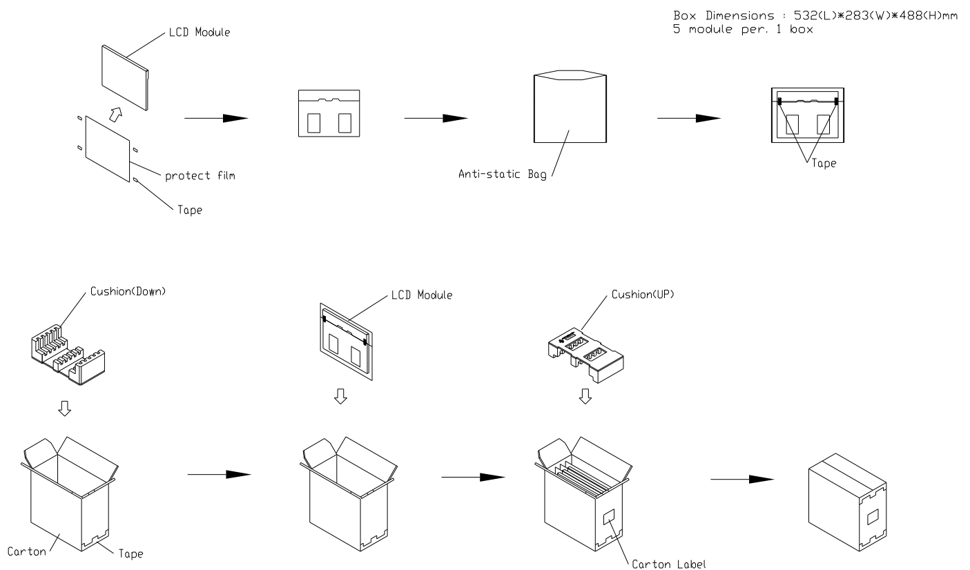
Figure. 7-1 Packing method
