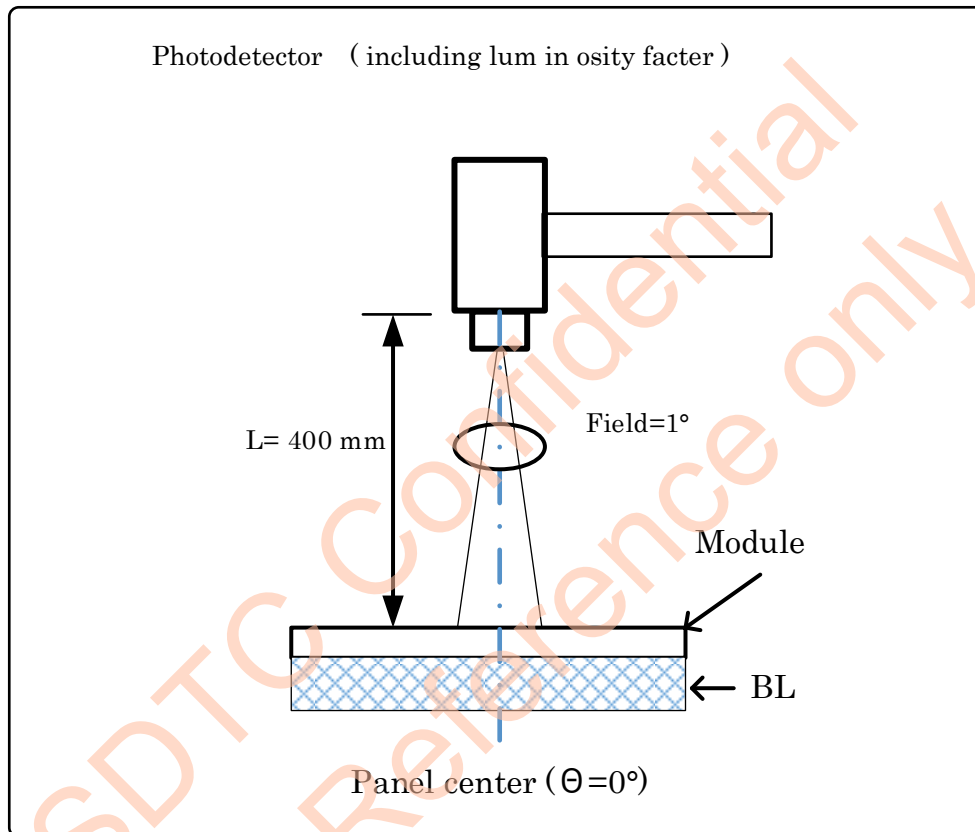
Figure 7-5 Measurement equipment (Transmissive mode)
