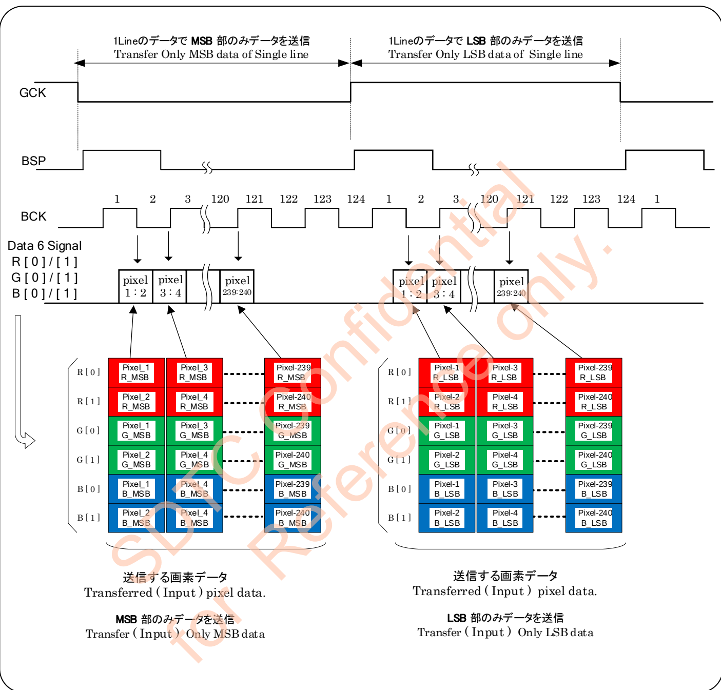
Figure 6-5-2 Horizontal Diagram
