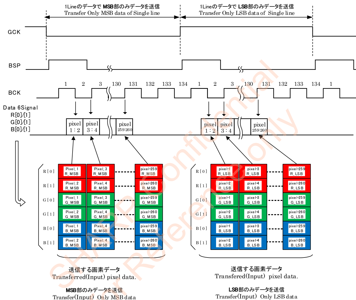
Figure 6-5-2 Horizontal Diagram
