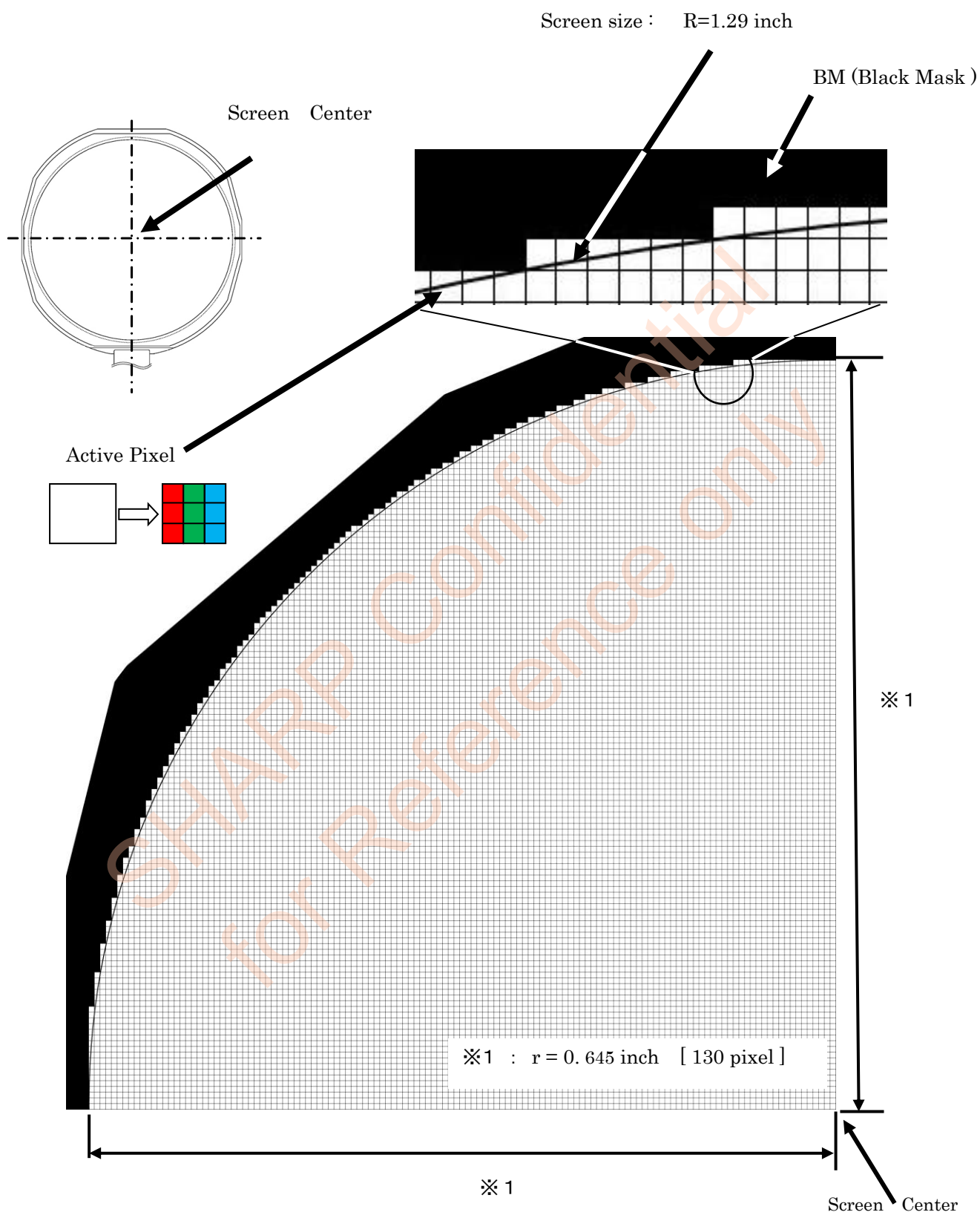
Figure 6-6-2 Data position 2
