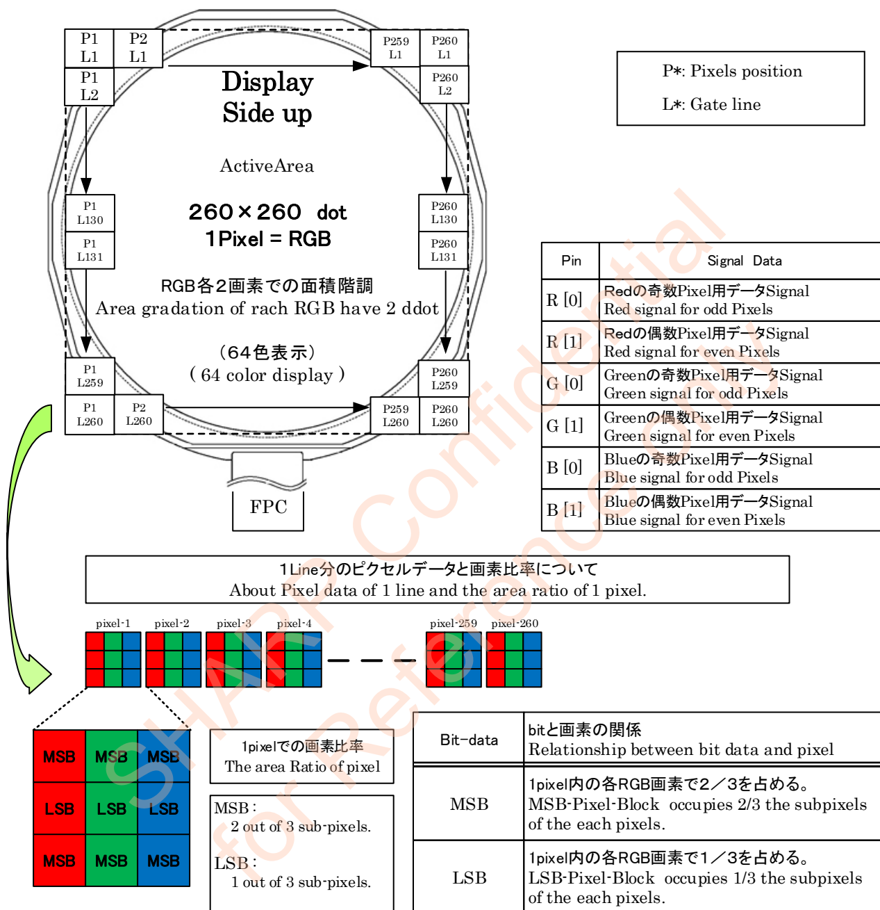
Figure 6-6-1 Data position 1
