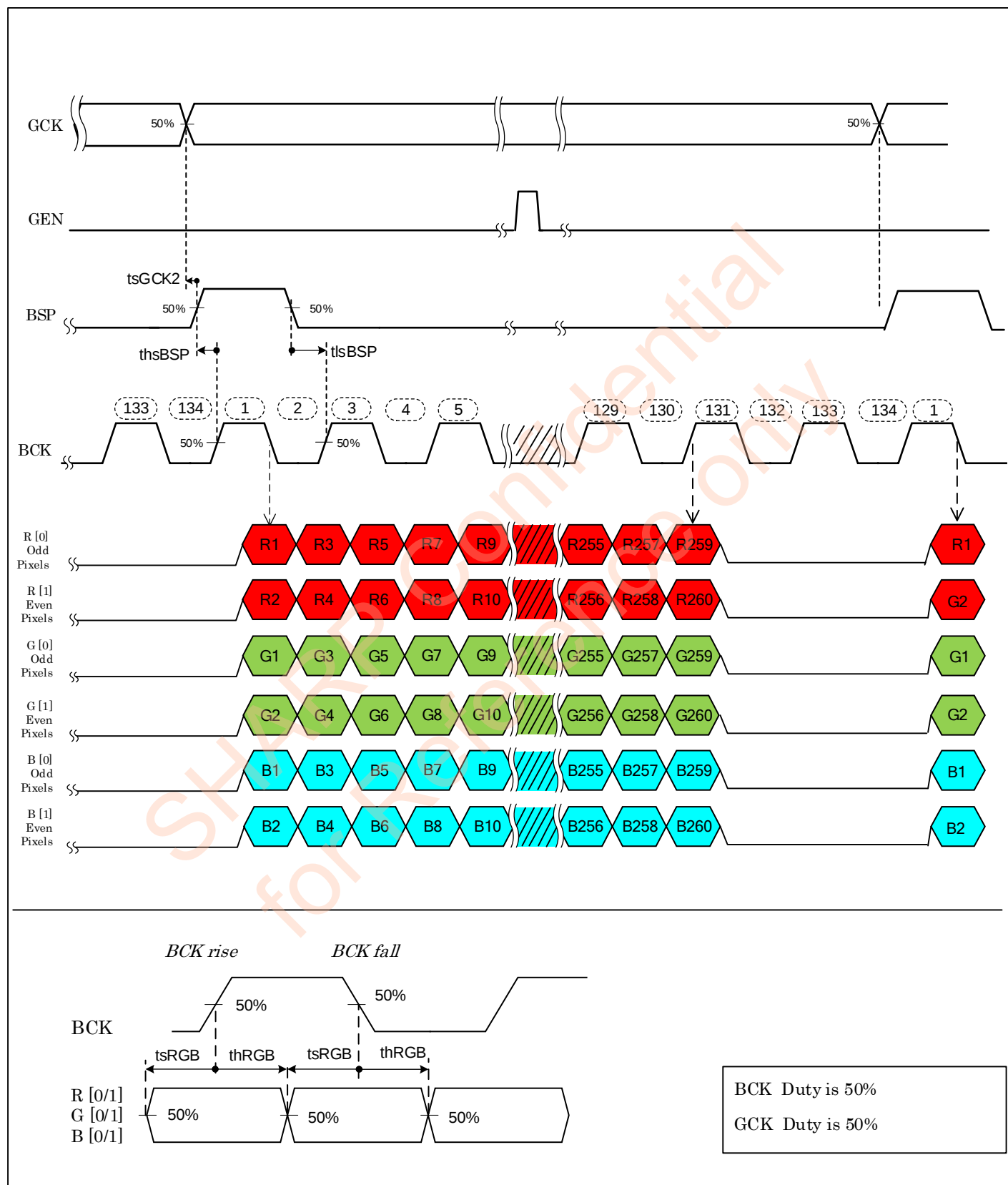
Figure 6-3-3 AC timing 3
