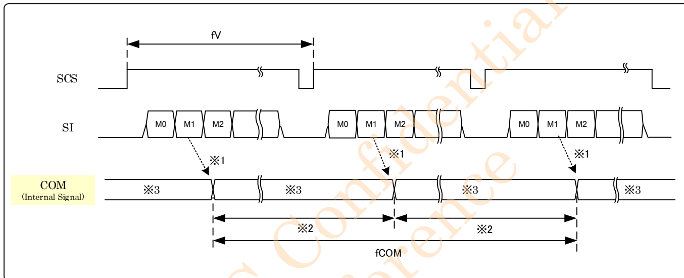
Figure 6-6-5 COM Inversion (EXTMODE=Lo)
