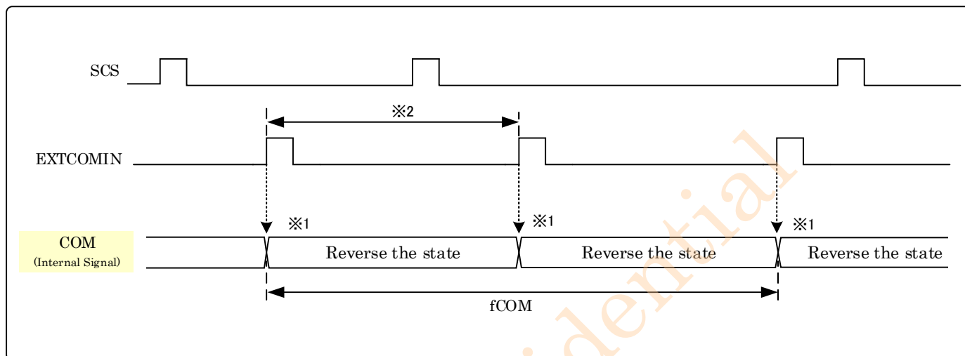
Figure 6-6-7 COM Inversion (EXTMODE=Hi)2
