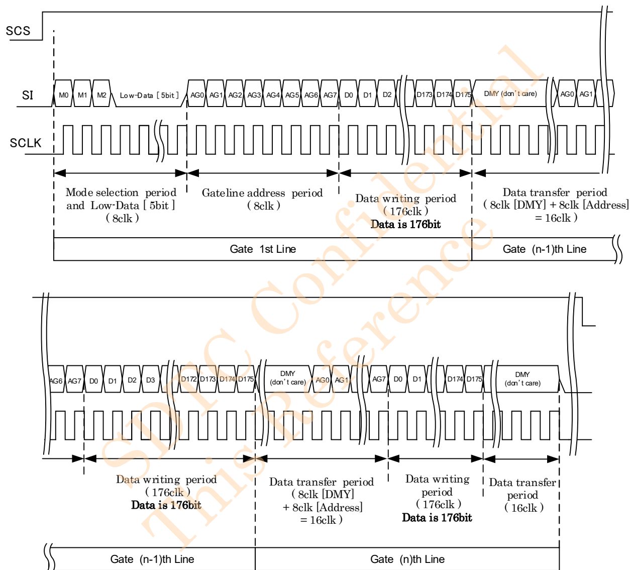
Figure 6-6-2 Data update mode by Multiple Lines
