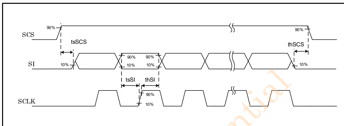
Figure 6-4-2 Signal Timing-2
