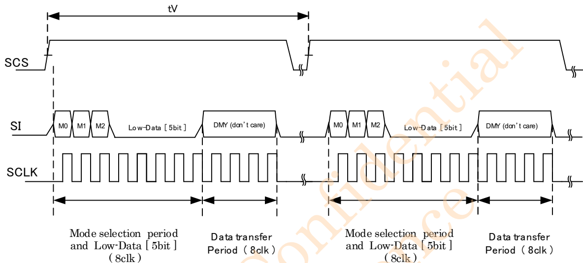
Figure 6-6-3 HOLD mode
