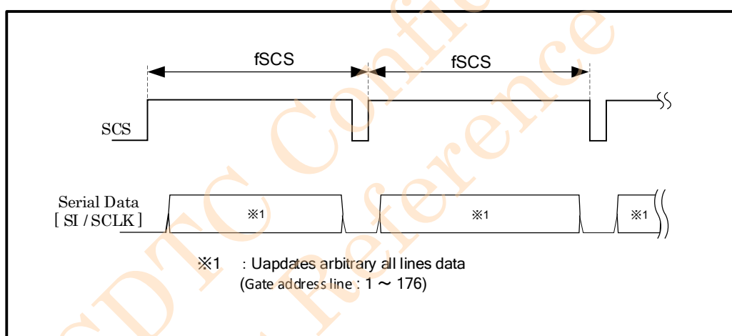
Figure 6-4-3 Signal Timing-3
