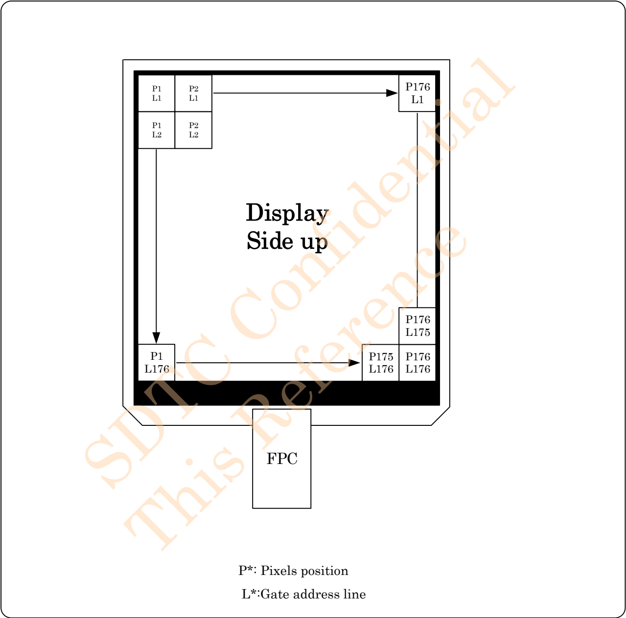
Figure 6-8-1 Data position
