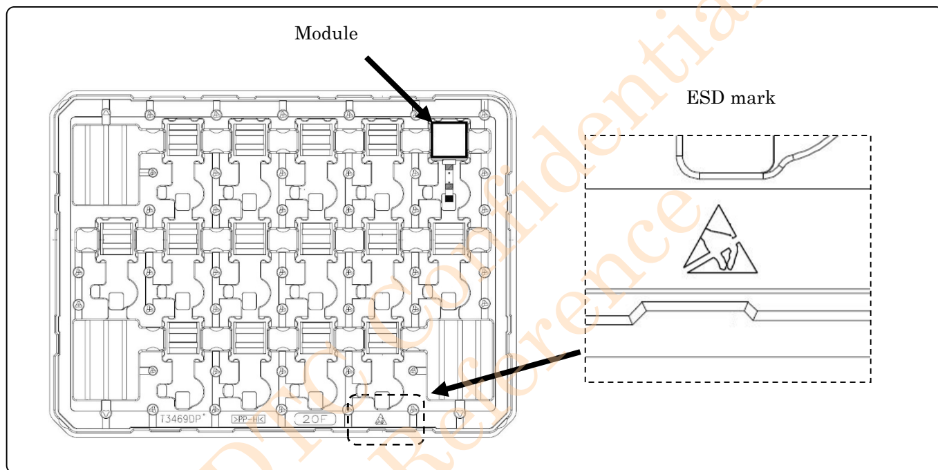
Figure. 12-2-1 Packaging Form 1
