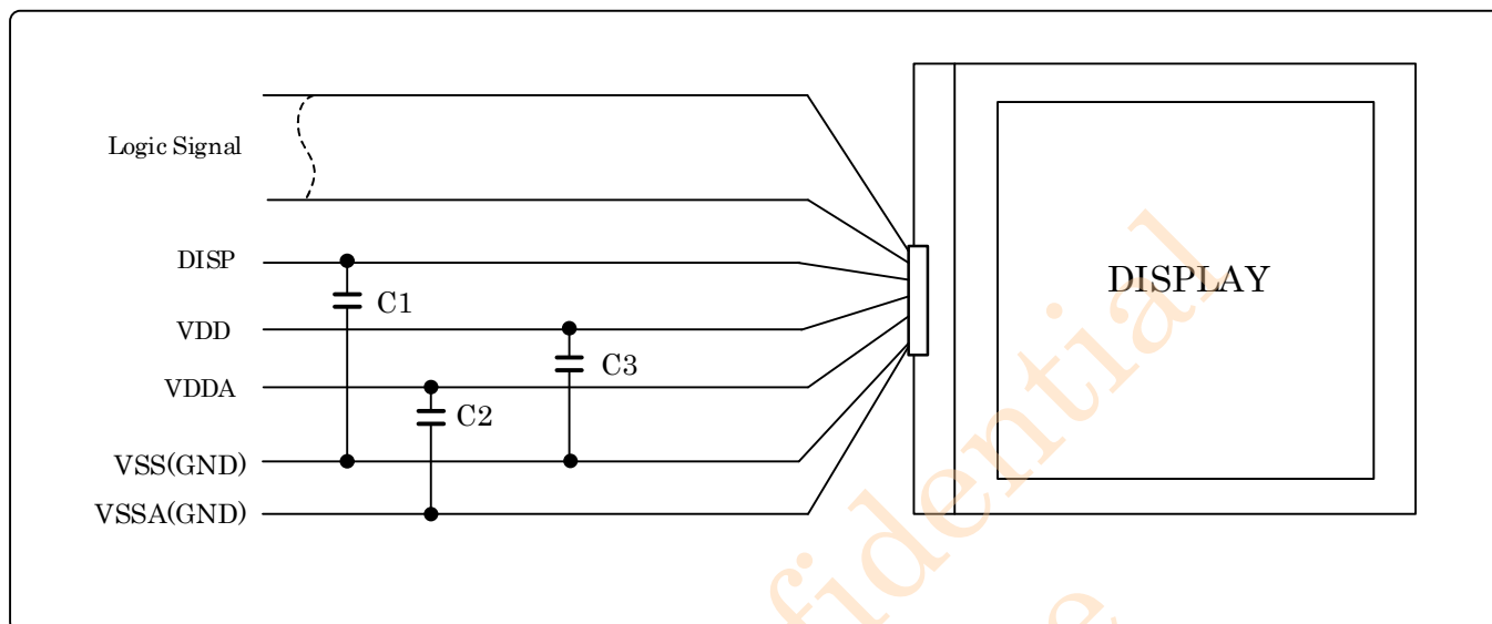
Figure 10-1 External capacitor recommendation capacity value
