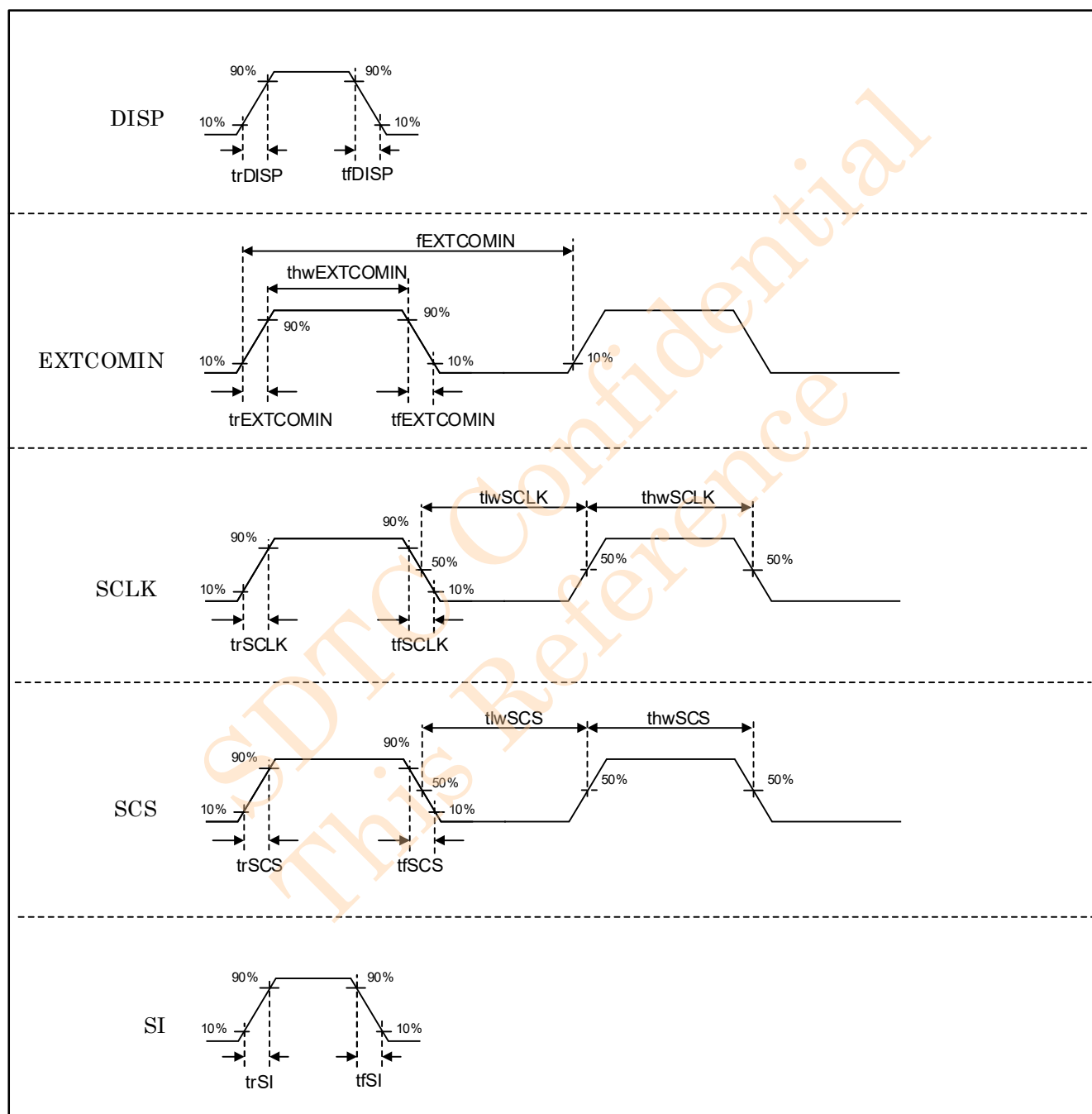
Figure 6-4-1 Signal Timing
