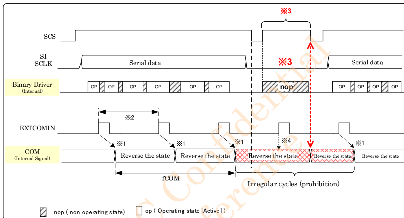
Figure 6-6-6 COM Inversion (EXTMODE=Hi) 1
