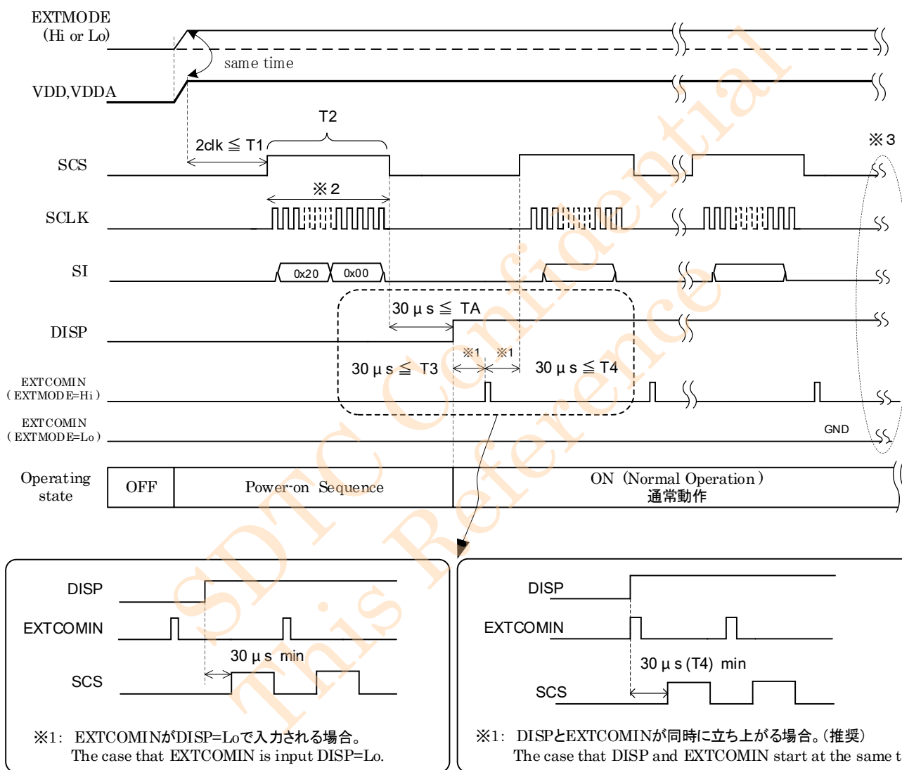
Figure 6-2-1 Power supply sequence
