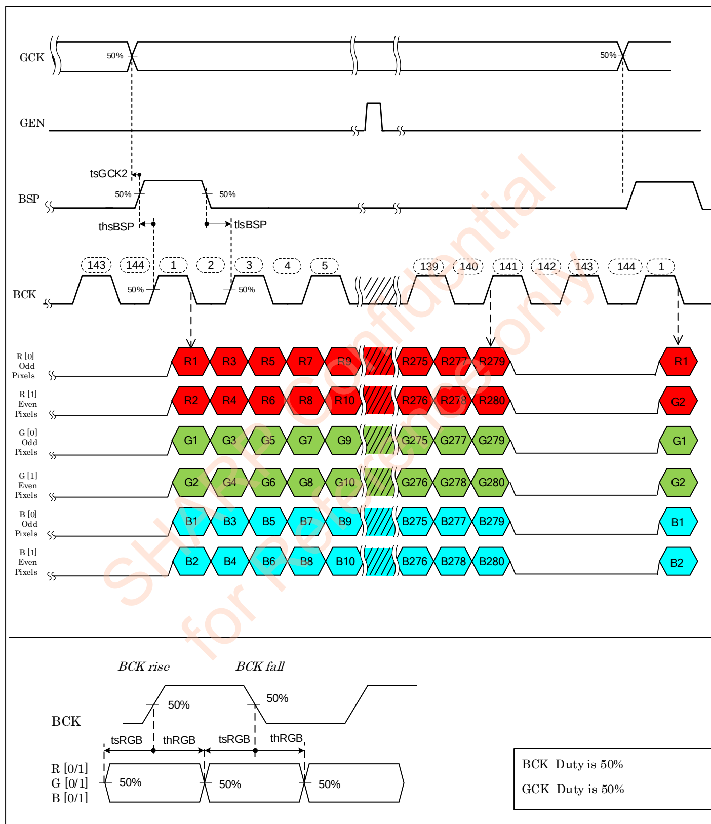
Figure 6-3-3 AC timing 3
