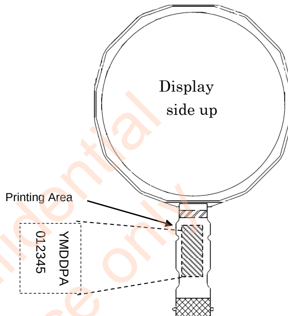
Figure. 11-1-1 Lot number printing position (top view not to scale)
