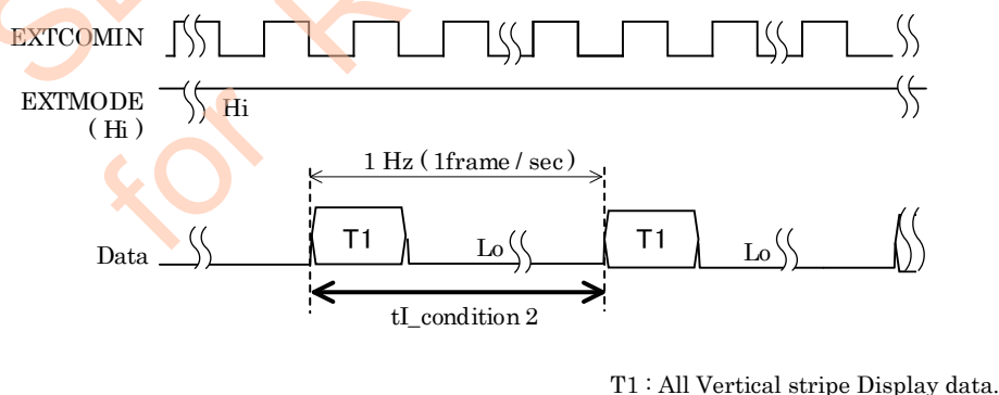
Figure 6-4-2 Current measurement 2
