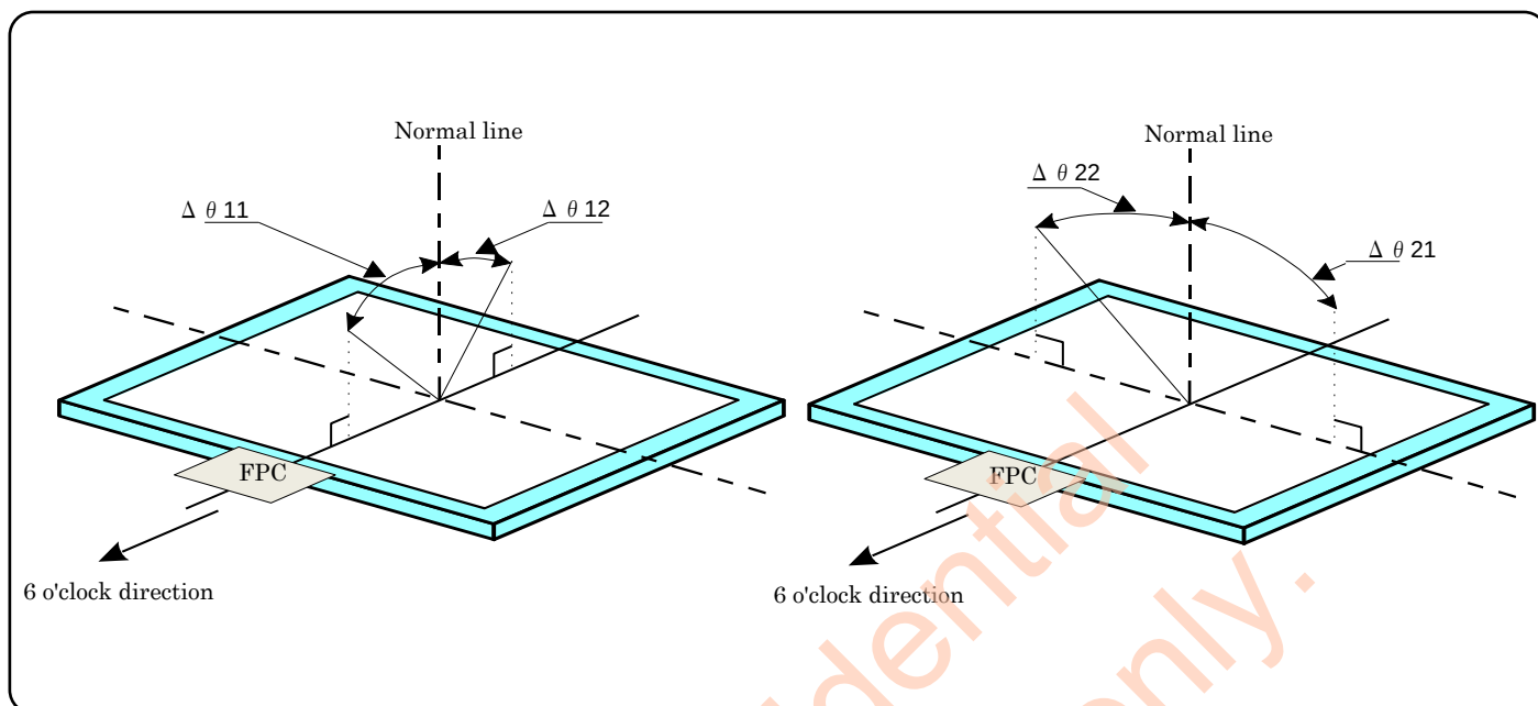
Figure 7-1 Definition of Viewing Angle
