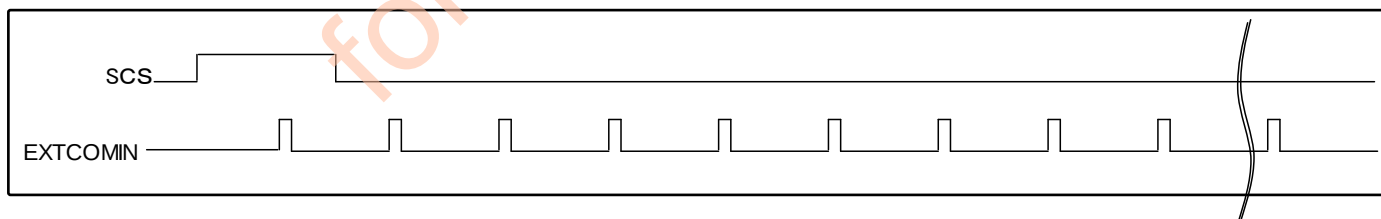
Figure 6-5-3 EXTCOMIN Signal 2
