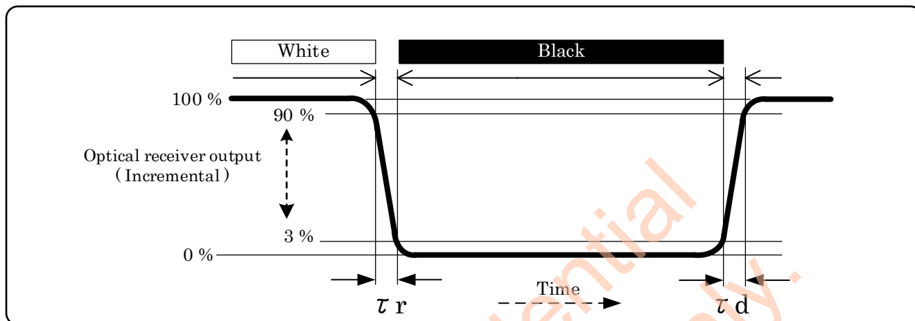
Figure 7-4 Response time
