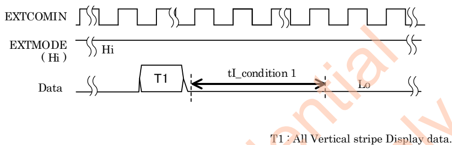
Figure 6-4-1 Current measurement 1
