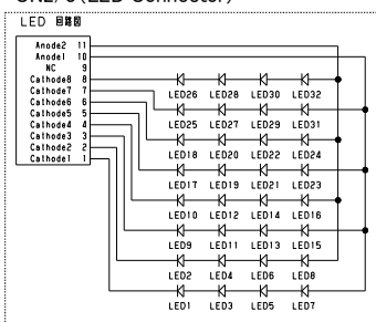
CN2/3(LED Connector)
