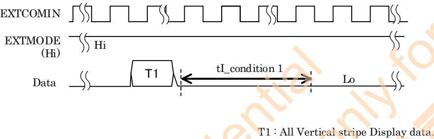
Figure 6-4-1 Current measurement 1
