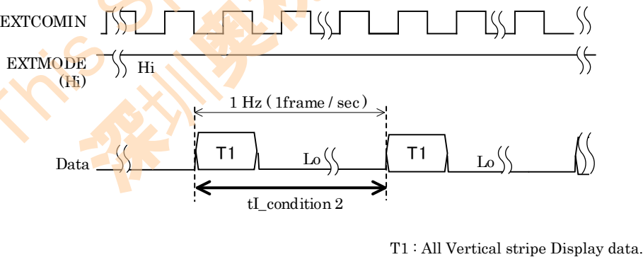
Figure 6-4-2 Current measurement 2
