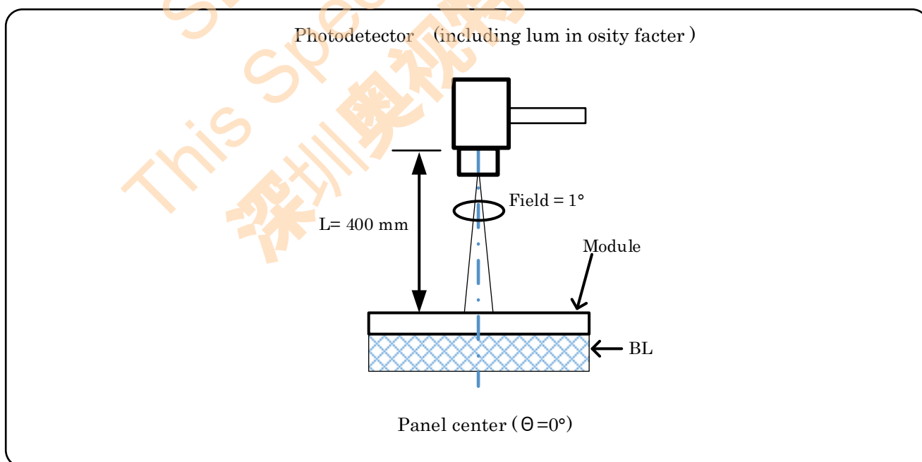
Figure 7-5 Measuring setup for Luminance
