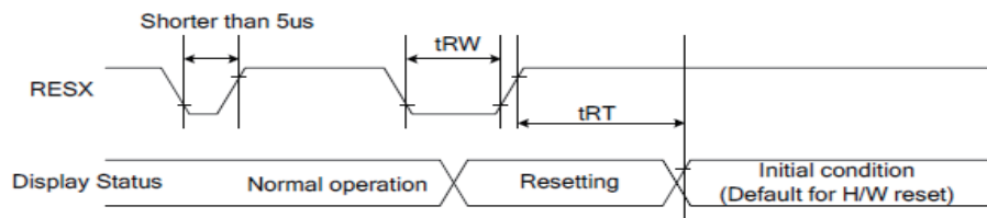
Figure 126: Reset Timing
