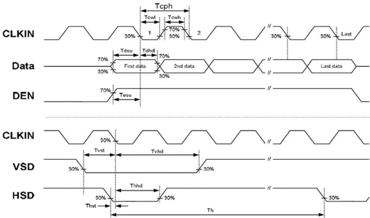
Figure 5.2.1 Input clock and data timing diagram
