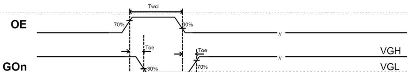
Figure 5.2.1 Gate driver input timing
