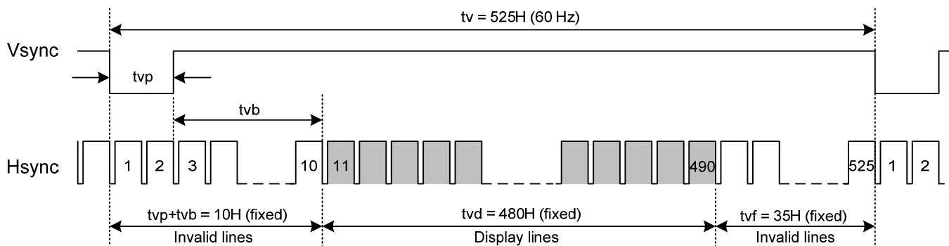
Fig. 9.2 Vertical Timing
