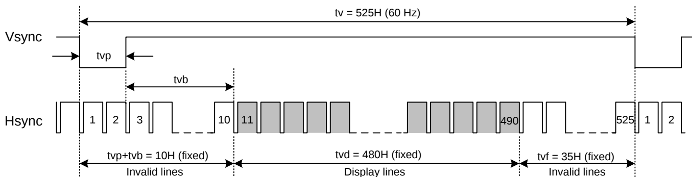
Fig. 9.2 Vertical Timing
