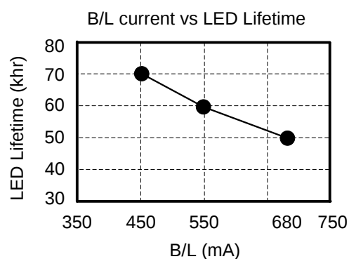
Fig 5.3 LED Current v.s. Lifetime
