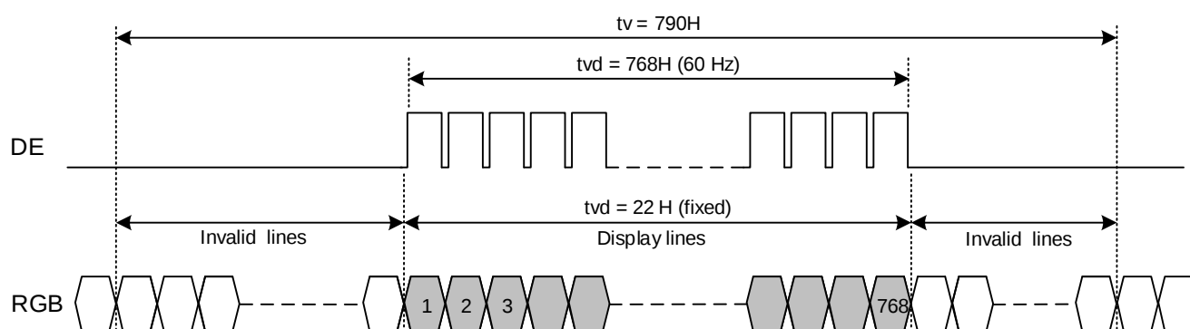
Fig. 8.2 Vertical Timing
