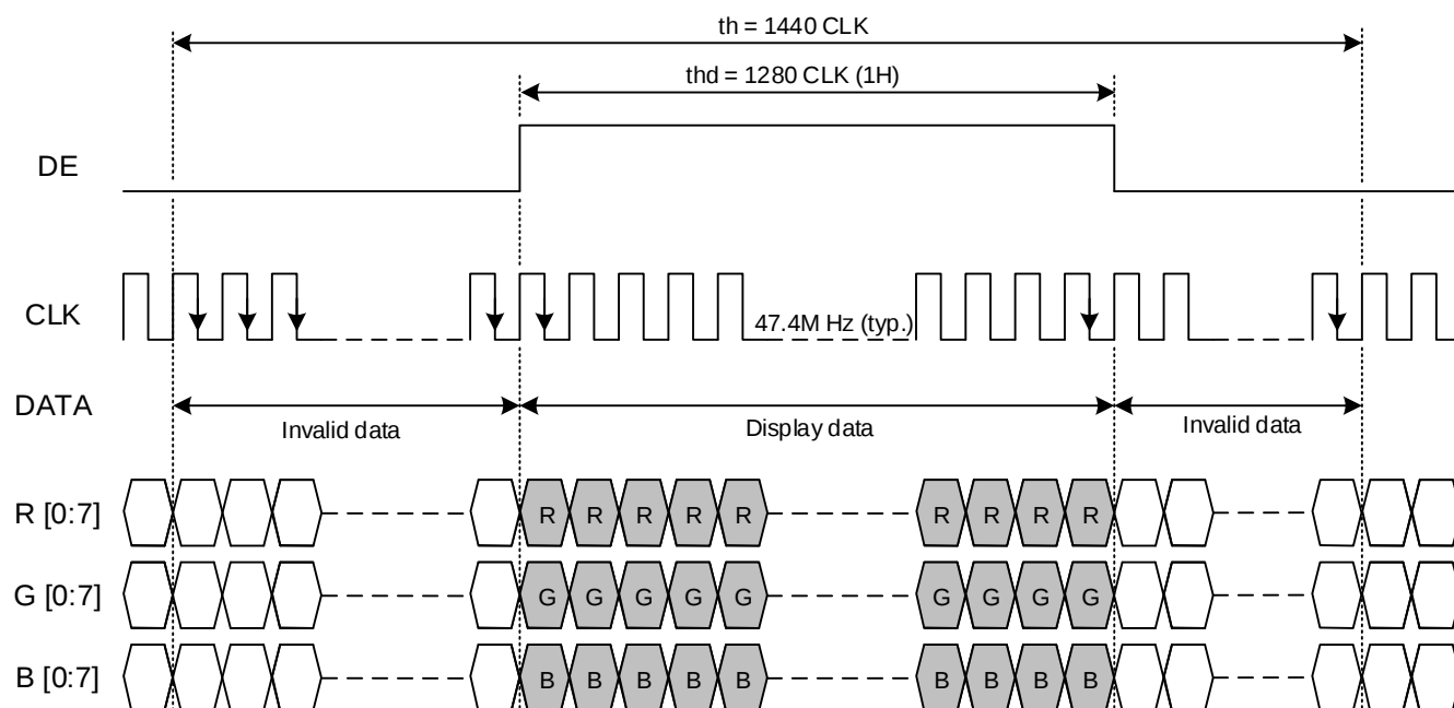
Fig. 8.1 Horizontal Timing
