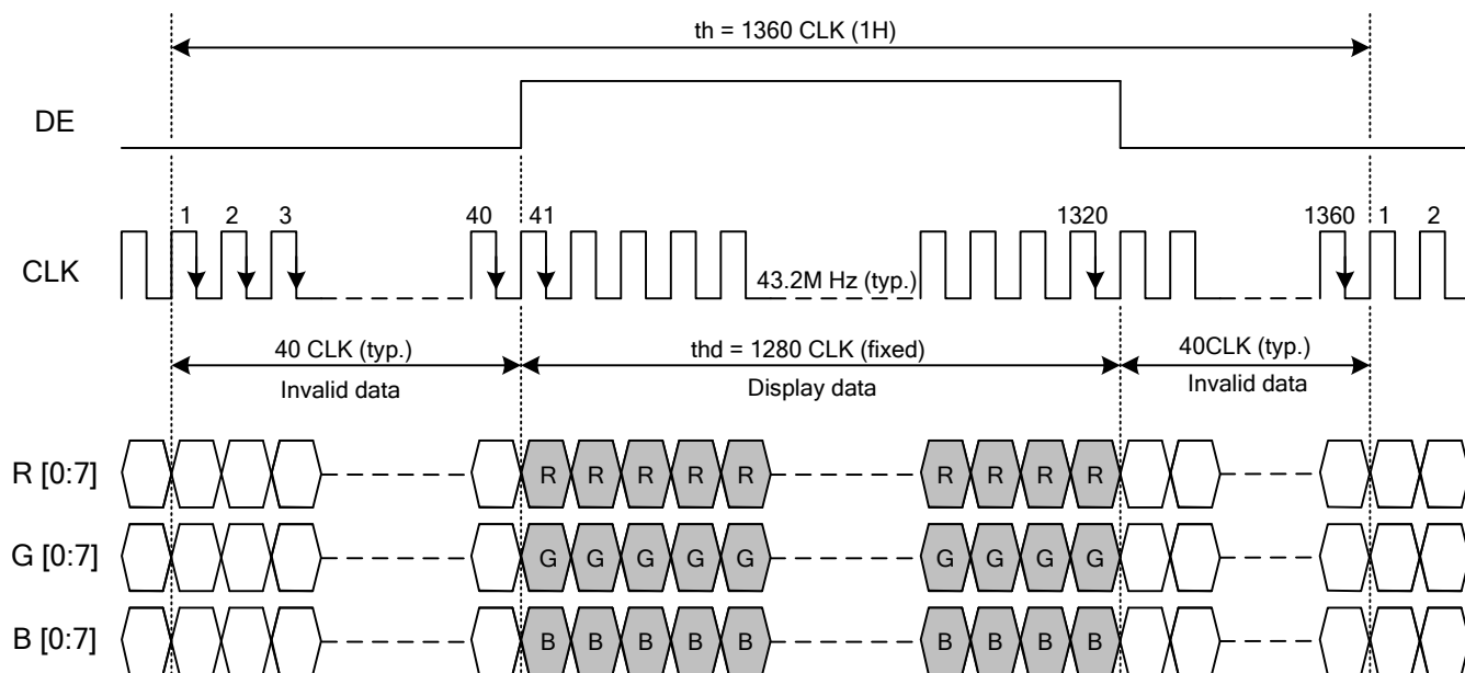
Fig. 9.1 Horizontal Timing
